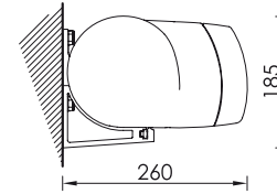
Montaggio a parete Wall installation
